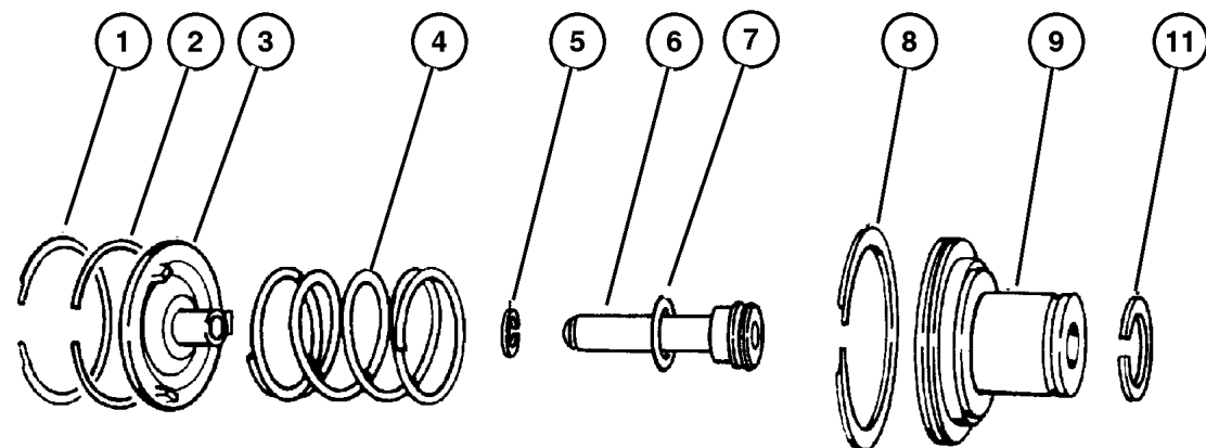
KICKDOWN SERVO
