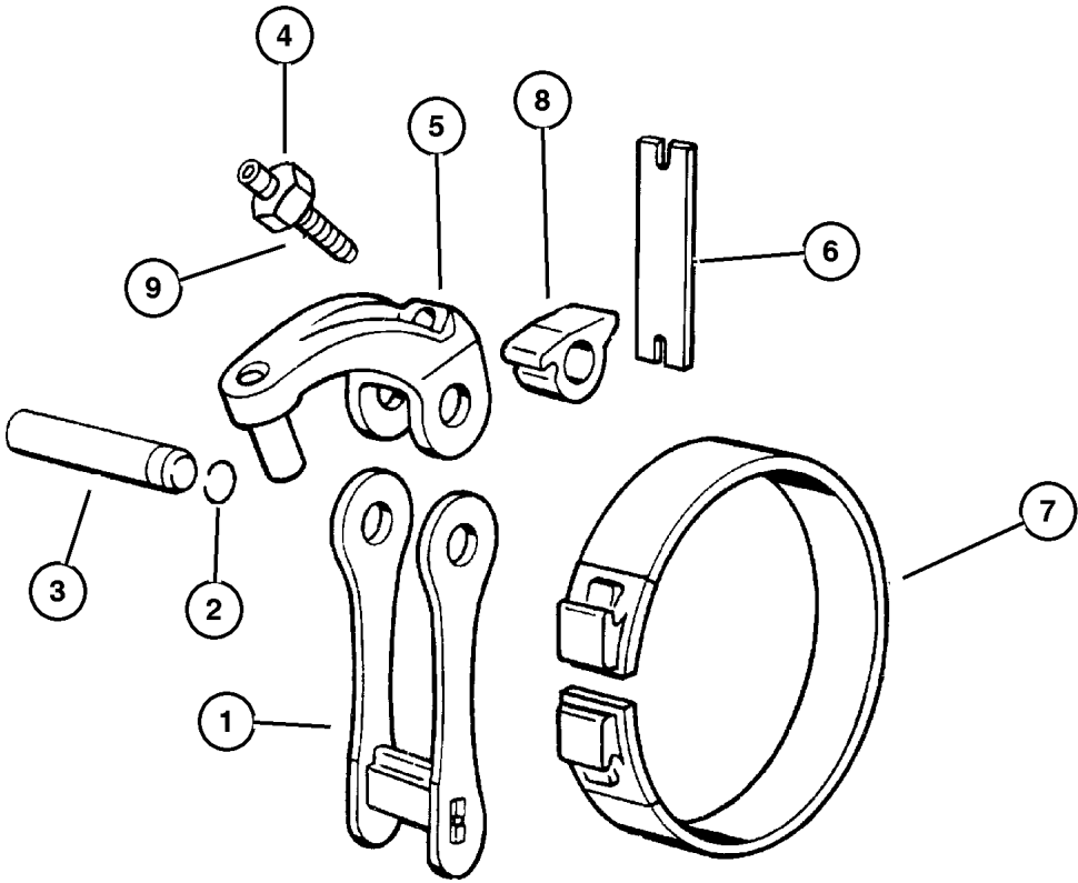
REVERSE BAND
