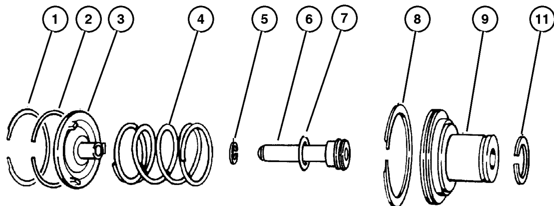
KICKDOWN SERVO
