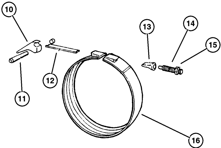
KICKDOWN BAND
