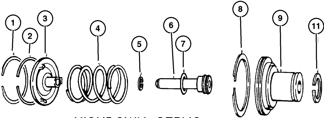
KICKDOWN SERVO
