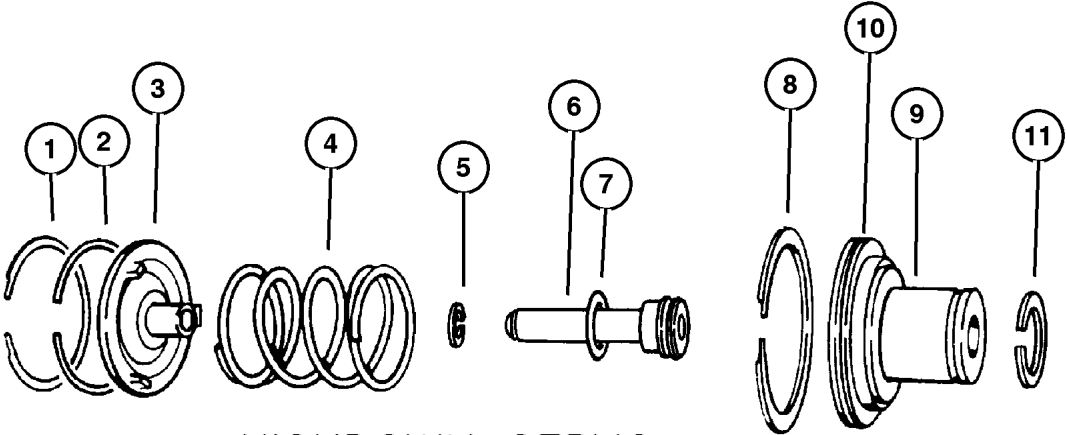
KICKDOWN SERVO
