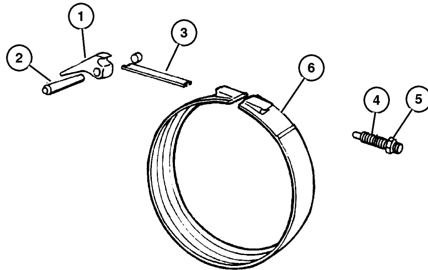
KICKDOWN BAND
