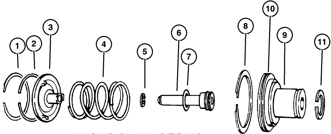
KICKDOWN SERVO
