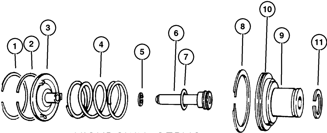
KICKDOWN SERVO
