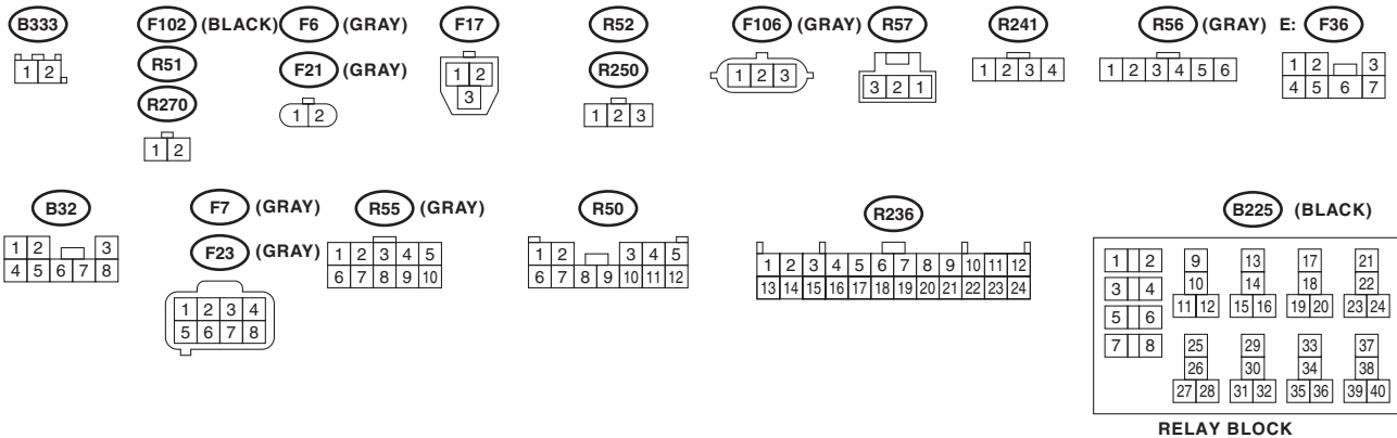
RELAY BLOCK
