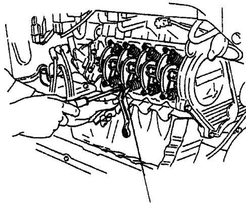
Thickness Gage
