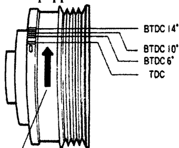
Engine Rotation
