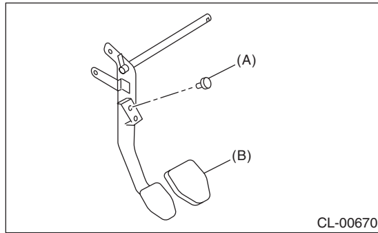
(A) Stopper (B) Clutch pedal pad
