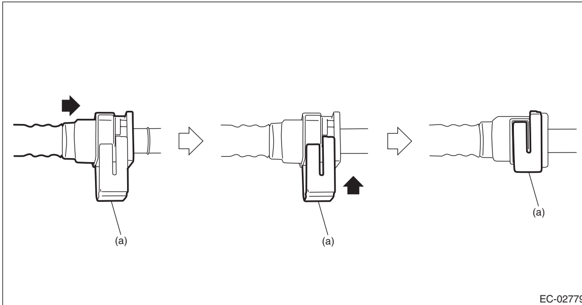
(a) Retainer
