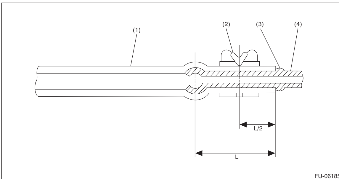
(1) Hose (2) Clip
