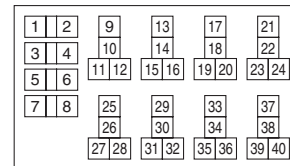
RELAY BLOCK
