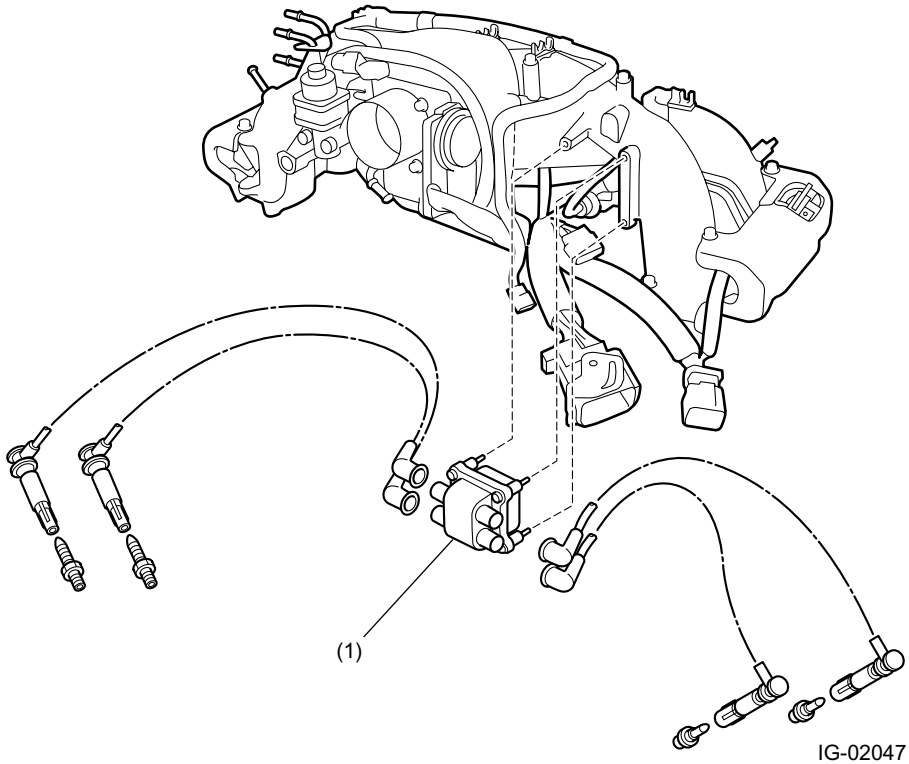
(1) Ignition coil and igniter assembly
