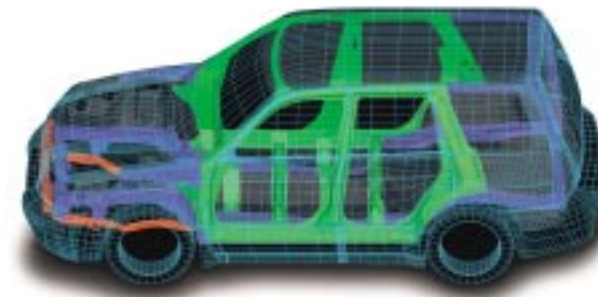
■ Ring-Shaped Reinforcement Frames ■ Sub frame ■ Chassis Reinforcement Frames
