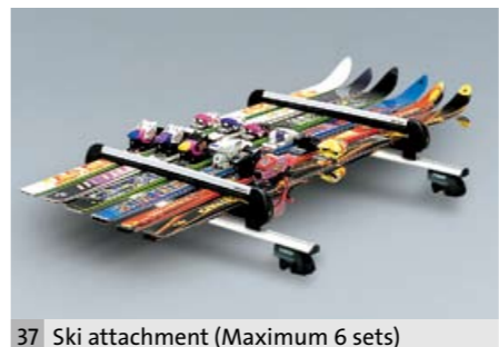
37 Ski attachment (Maximum 6 sets) E361EAG550 For 6 sets of skis or 4 snowboards. Usable width: 640 mm. *Aluminium carrier base required.
