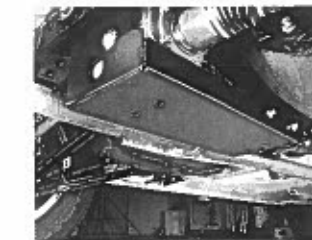
40 Differential guard
