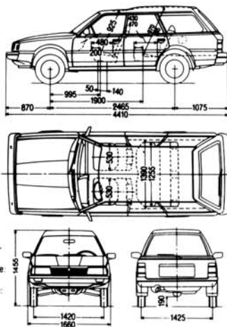
Super-Station 1800 Allrad
