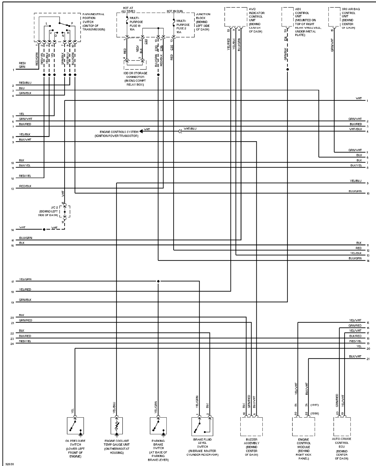
Instrument Cluster Circuit (2 of 3)
