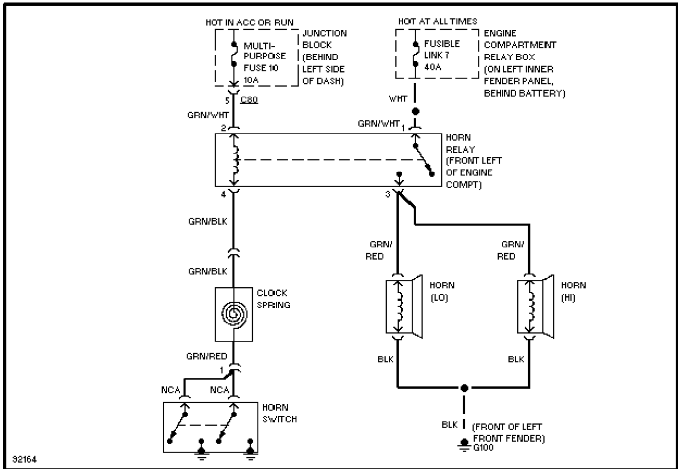
Horn Circuit
