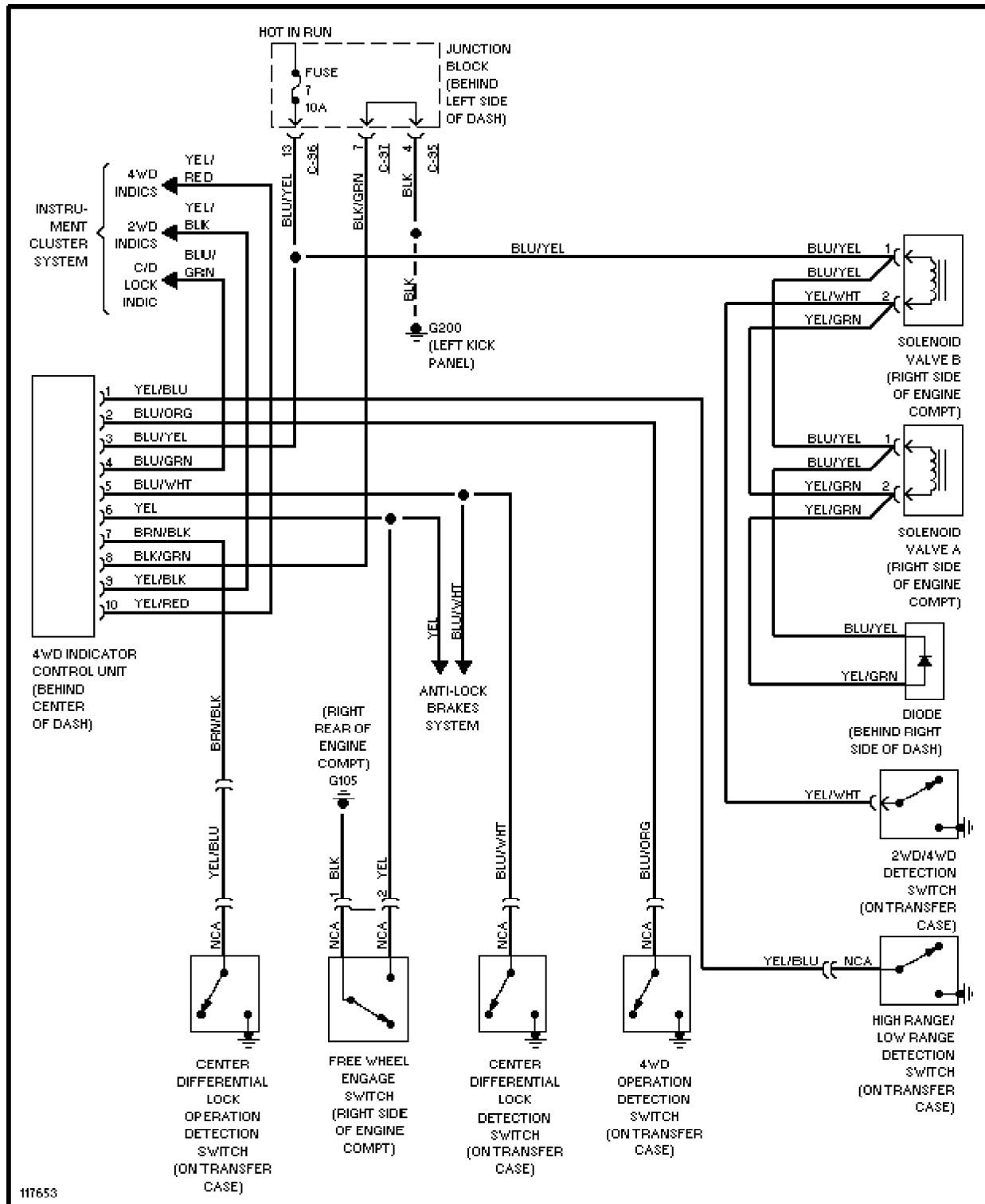
4WD Circuit, W/ Active Trac
