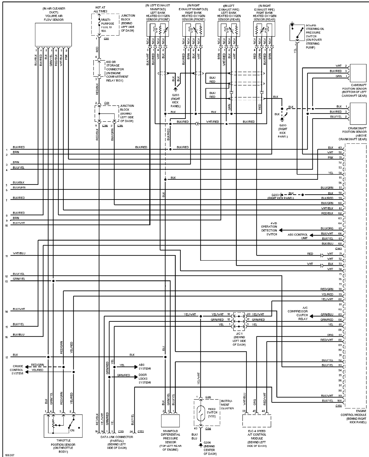
3.5L, Engine Performance Circuits, California (3 of 3)
