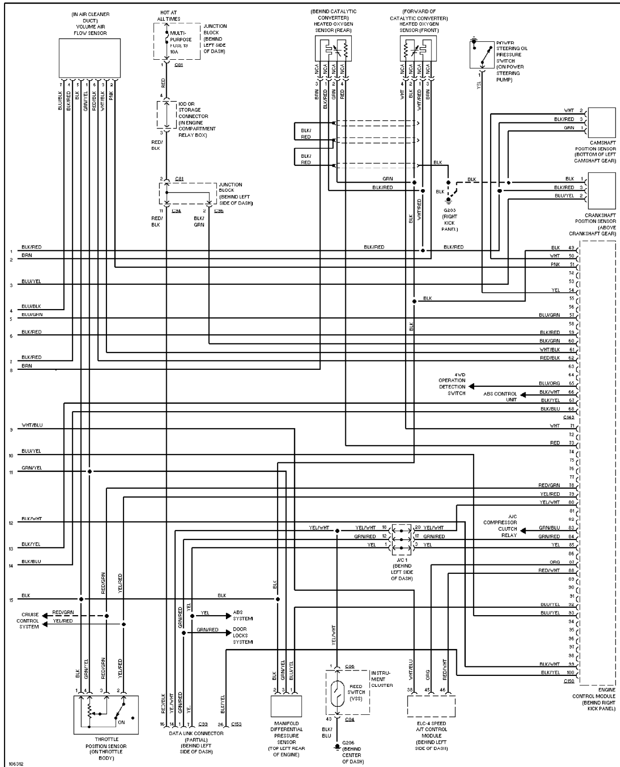
3.5L, Engine Performance Circuits, Federal (3 of 3)
