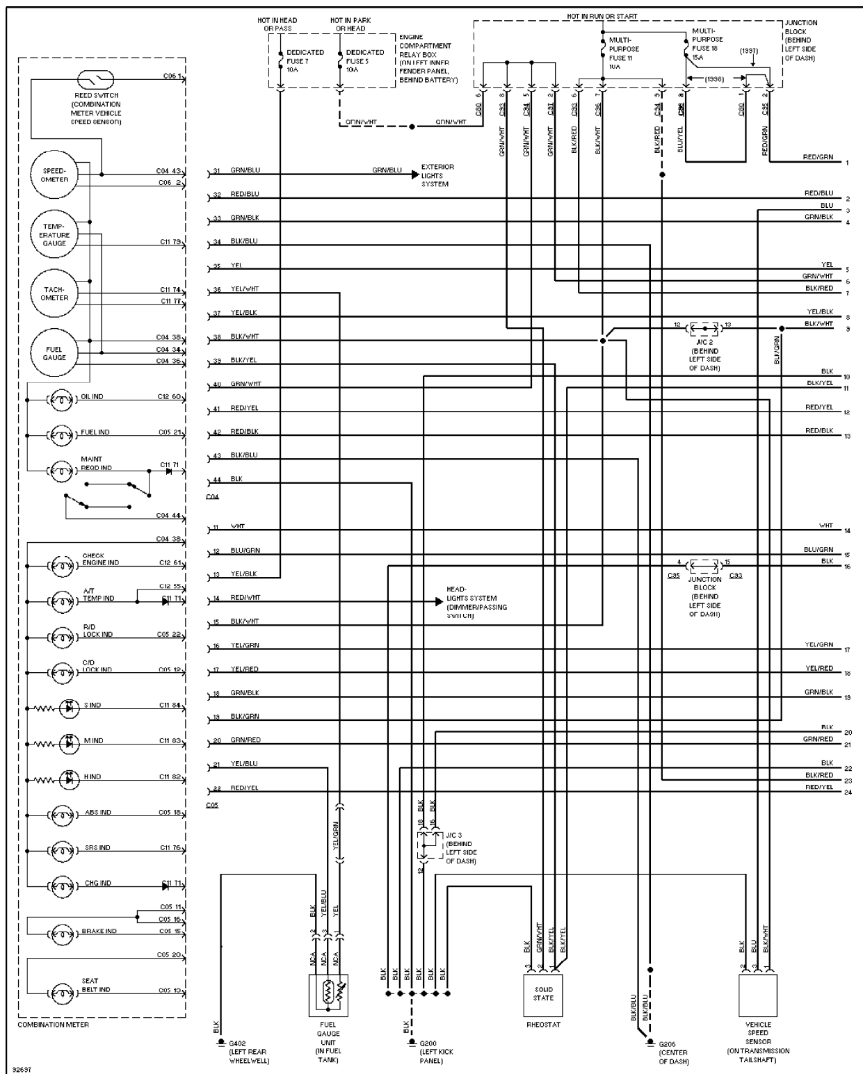
Instrument Cluster Circuit (1 of 3)
