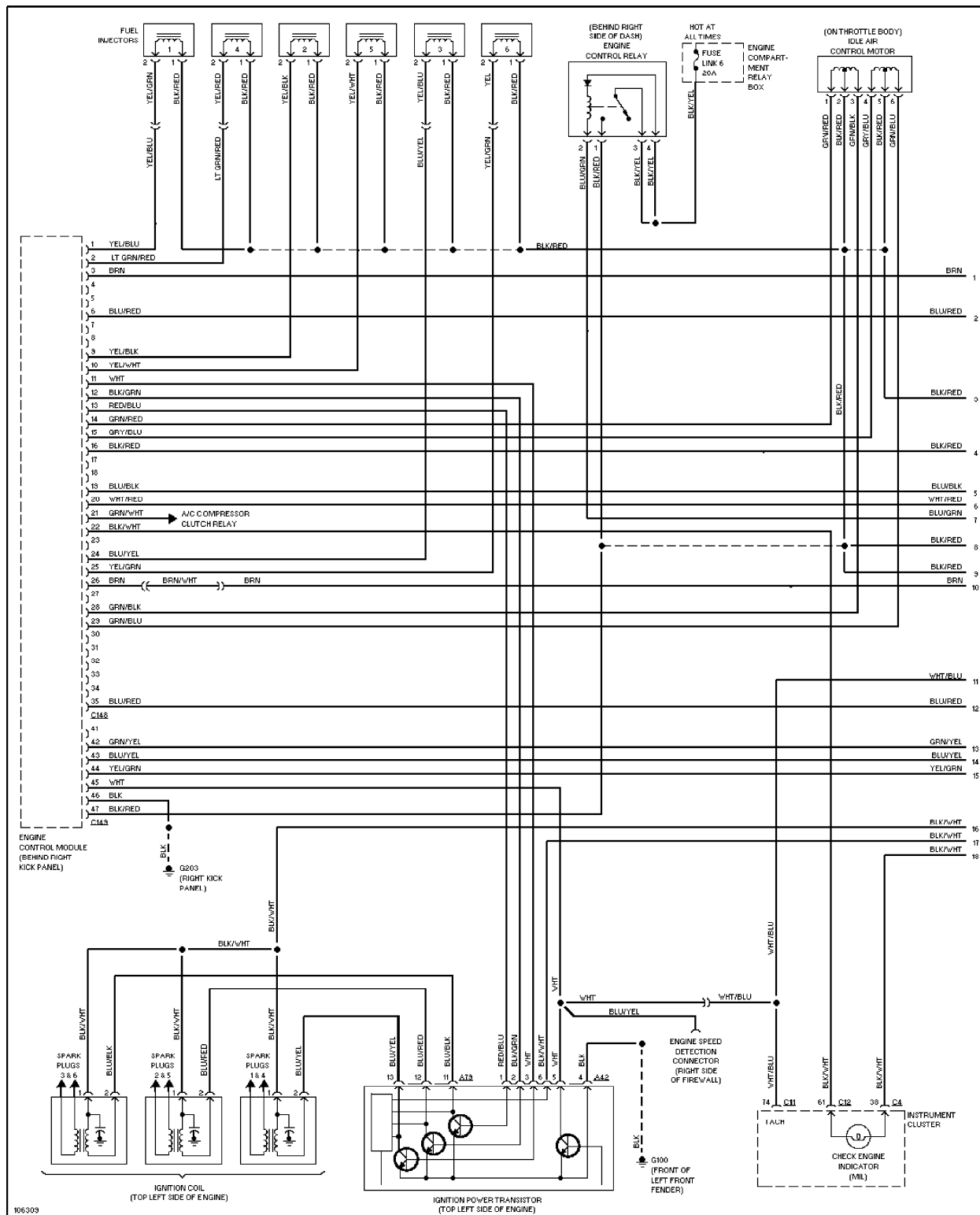
3.5L, Engine Performance Circuits, Federal (1 of 3)
