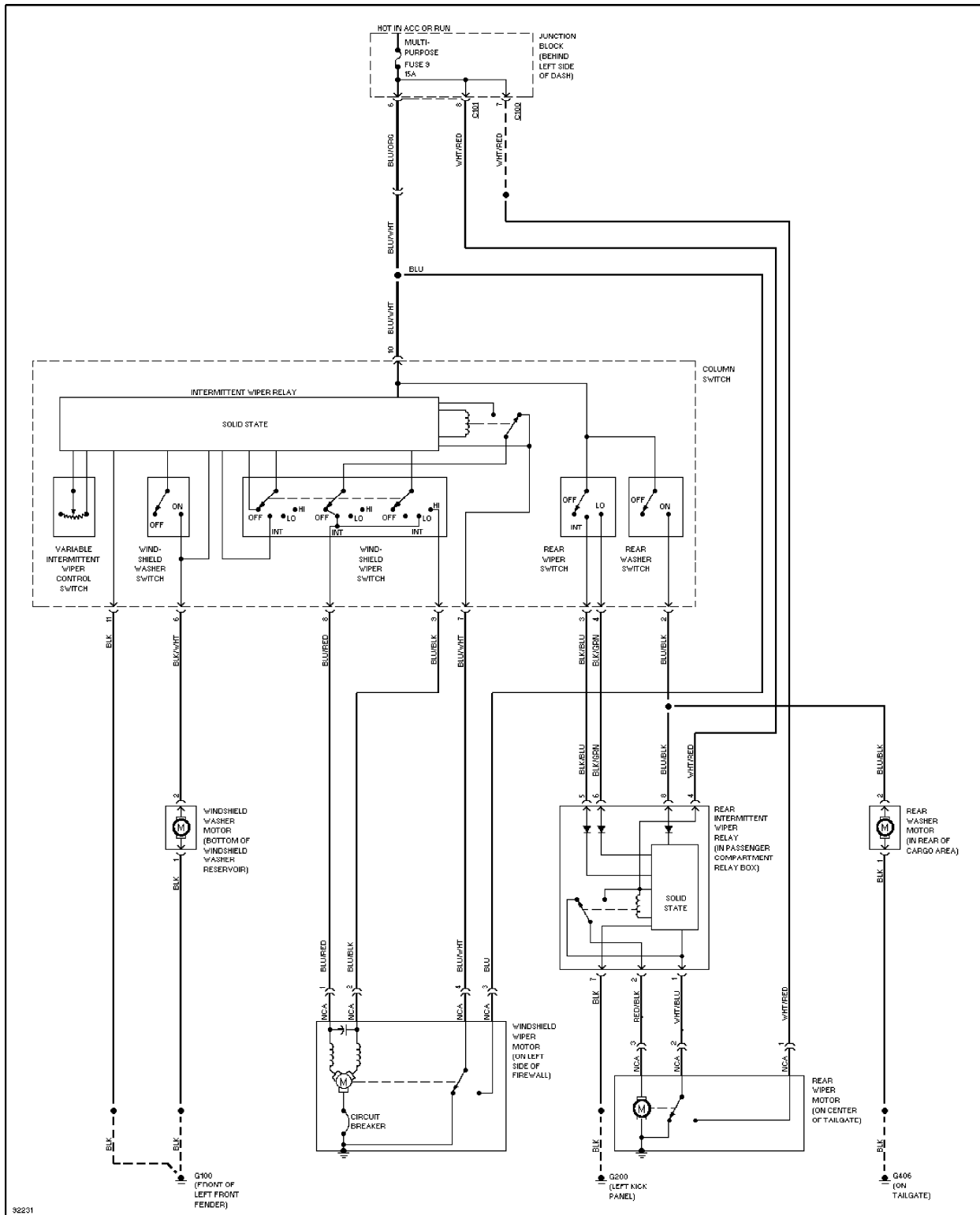
Wiper/Washer Circuit
