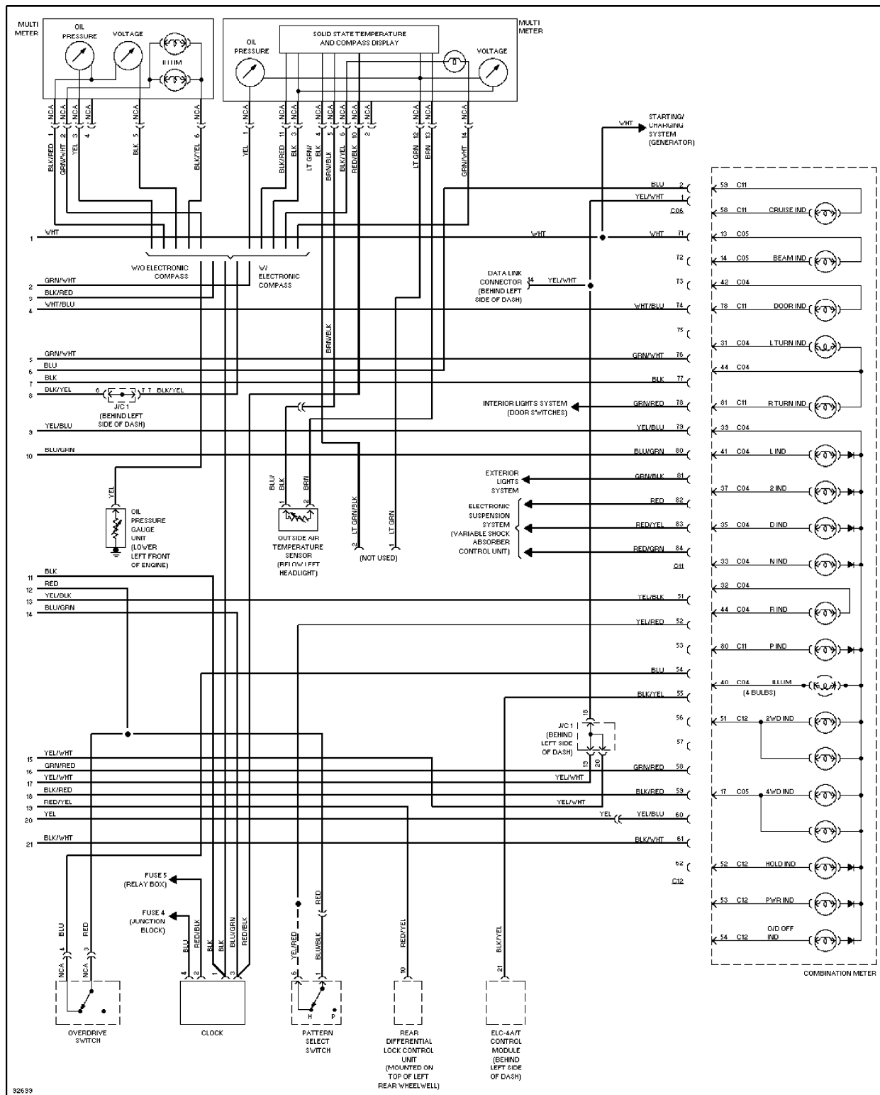
Instrument Cluster Circuit (3 of 3)
