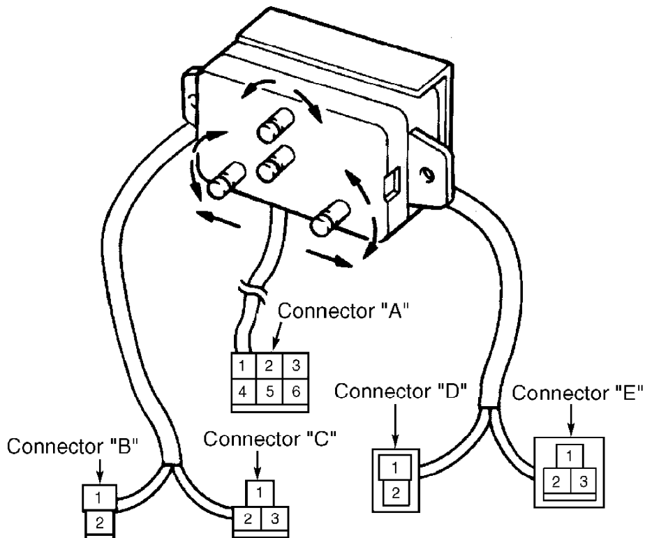
96B06432 Fig. 6: Identifying Power Seat Switch Terminals (Montero) Courtesy of Mitsubishi Motor Sales of America
