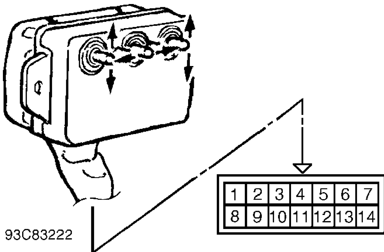
Fig. 4: Identifying Power Seat Switch Terminals (Eclipse & 3000GT) Courtesy of Mitsubishi Motor Sales of America
