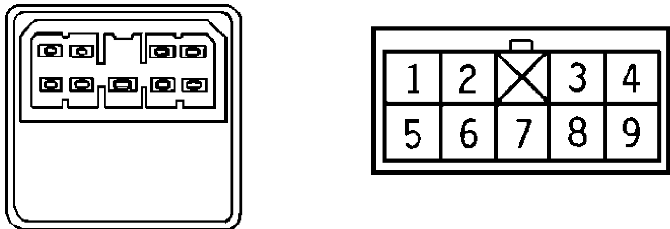
Fig. 7: Identifying Power Mirror Switch Terminals (Eclipse) Courtesy of Mitsubishi Motor Sales of America
