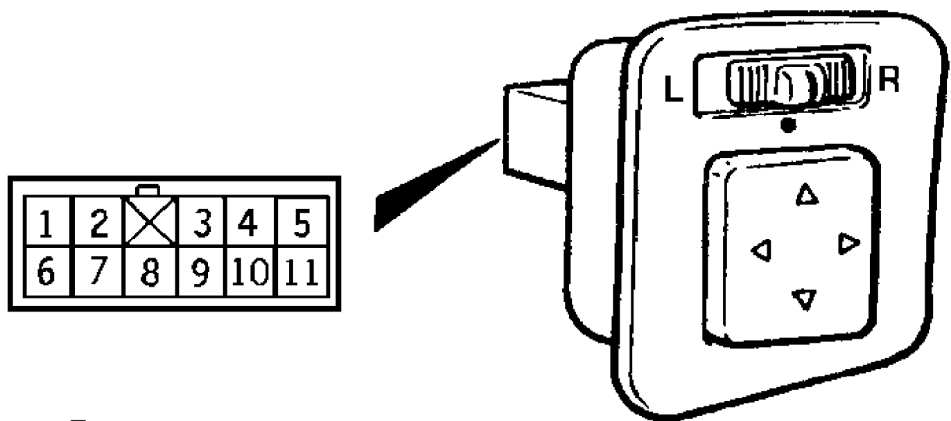
Fig. 7: Identifying Power Mirror Switch Terminals (Eclipse) Courtesy of Mitsubishi Motor Sales of America
