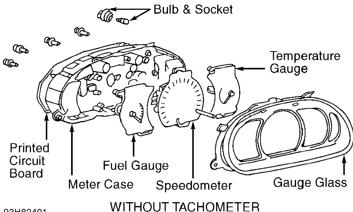
Fig. 42: Identifying Instrument Cluster Components (Mirage) Courtesy of Mitsubishi Motor Sales of America
