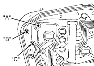
Fig. 24: Identifying Temperature Gauge Resistance Test Terminals (Mirage - With Tachometer)
