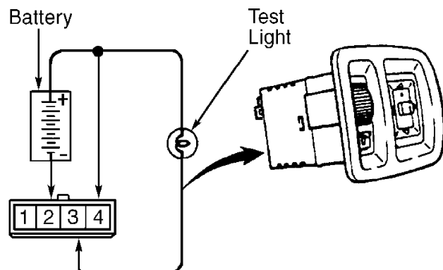
Fig. 38: Identifying Rheostat Connector Terminals (3000GT) Courtesy of Mitsubishi Motor Sales of America
