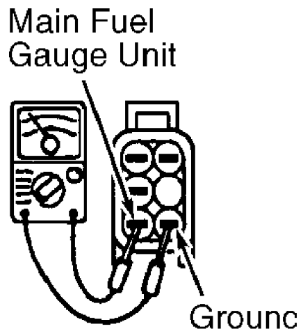
Fig. 4: Identifying Fuel Gauge Test Connections (Eclipse AWD - Main) Courtesy of Mitsubishi Motor Sales of America
