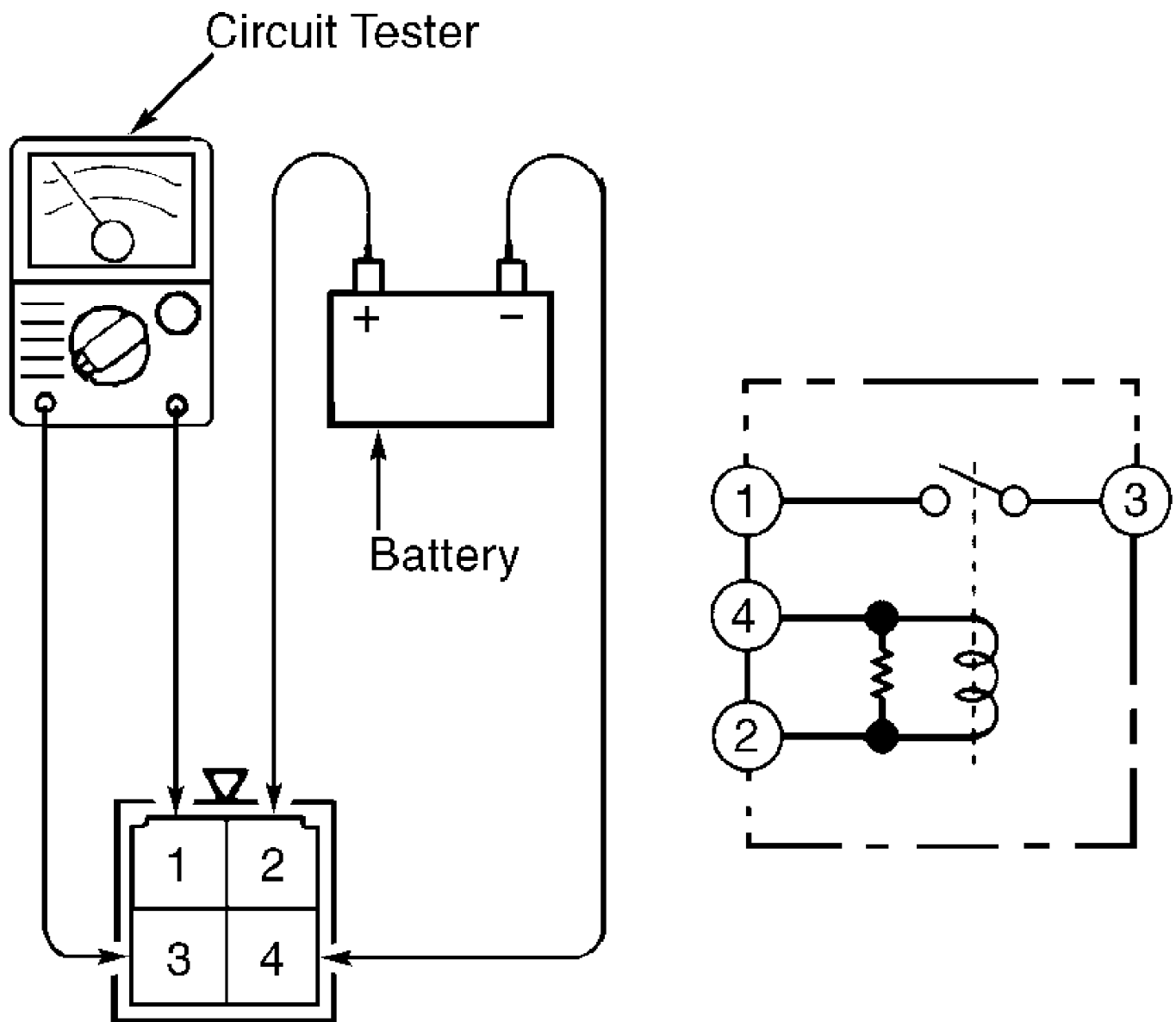
Fig. 9: Testing Electric Cooling Fan Relay (Montero, Montero Sport & 3000GT)
