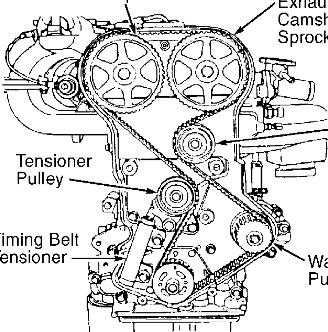
Fig. 3: Routing Timing/Water Pump Belt (Eclipse - 2.0L Non-Turbo) Courtesy of Mitsubishi Motor Sales of America.
