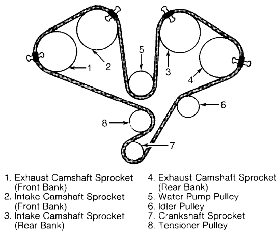
Fig. 6: Routing Timing/Water Pump Belt (3000GT - DOHC) Courtesy of Mitsubishi Motor Sales of America.
