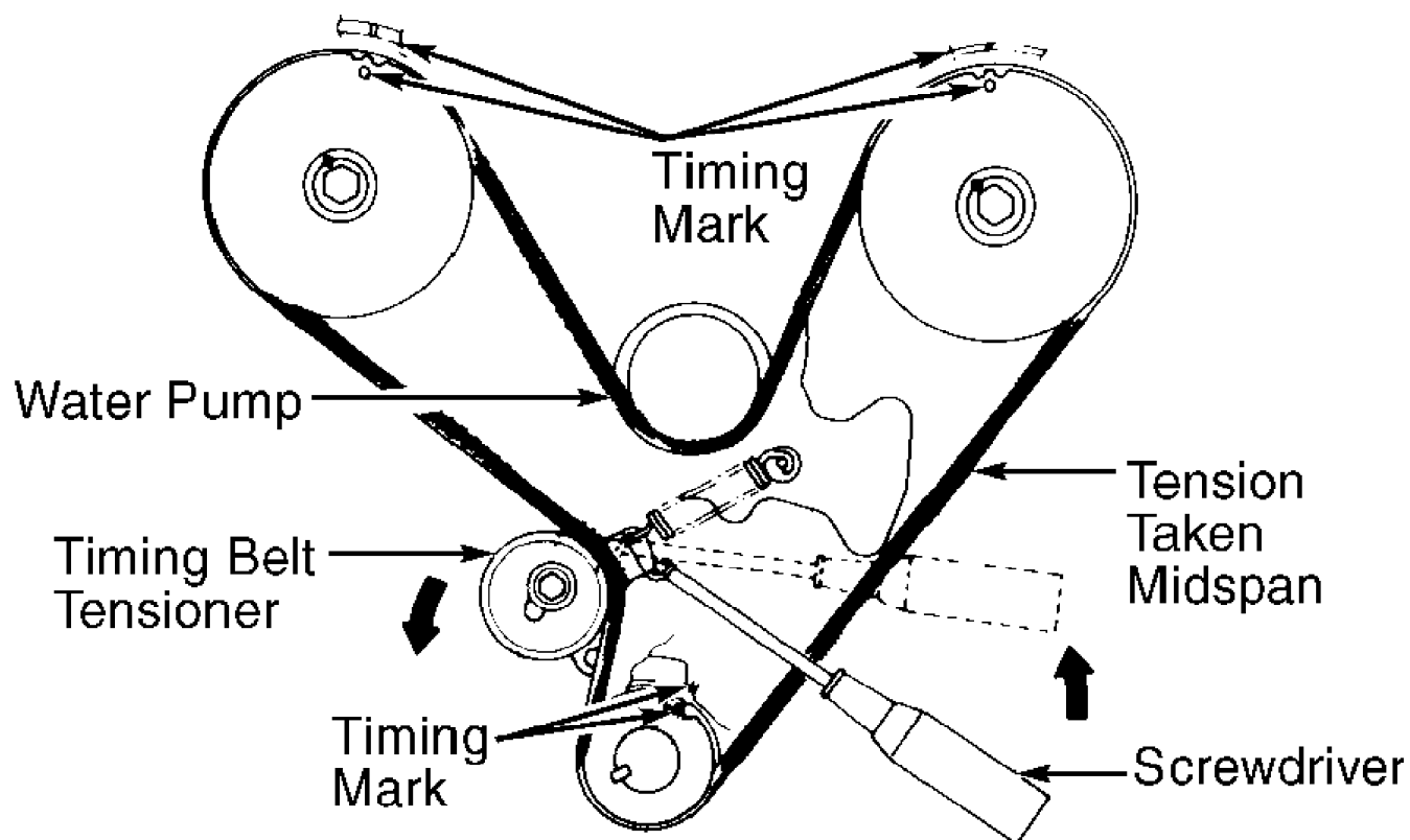
Fig. 1: Routing Timing/Water Pump Belt (Diamante & 3000GT SOHC) Courtesy of Mitsubishi Motor Sales of America.
