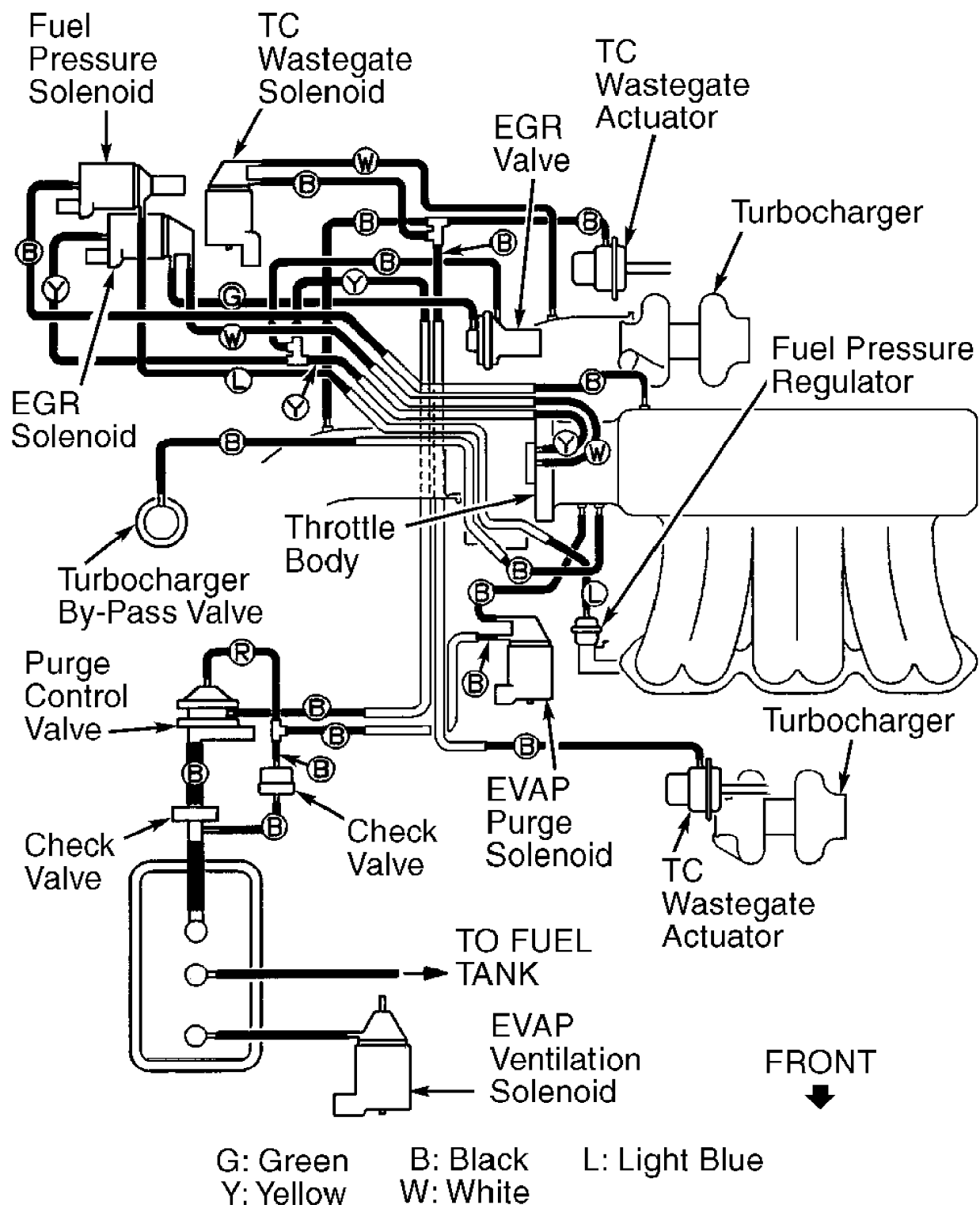
Fig. 16: Vacuum Diagram (3000GT DOHC Turbo) Courtesy of Mitsubishi Motor Sales of America
