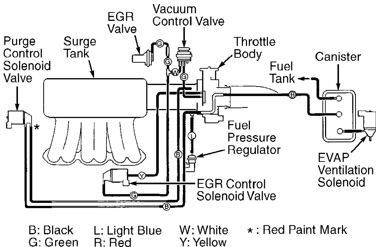
Fig. 1: Vacuum Diagram (Diamante) Courtesy of Mitsubishi Motor Sales of America
