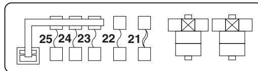
Relay box connected directly to ETACS-ECU
