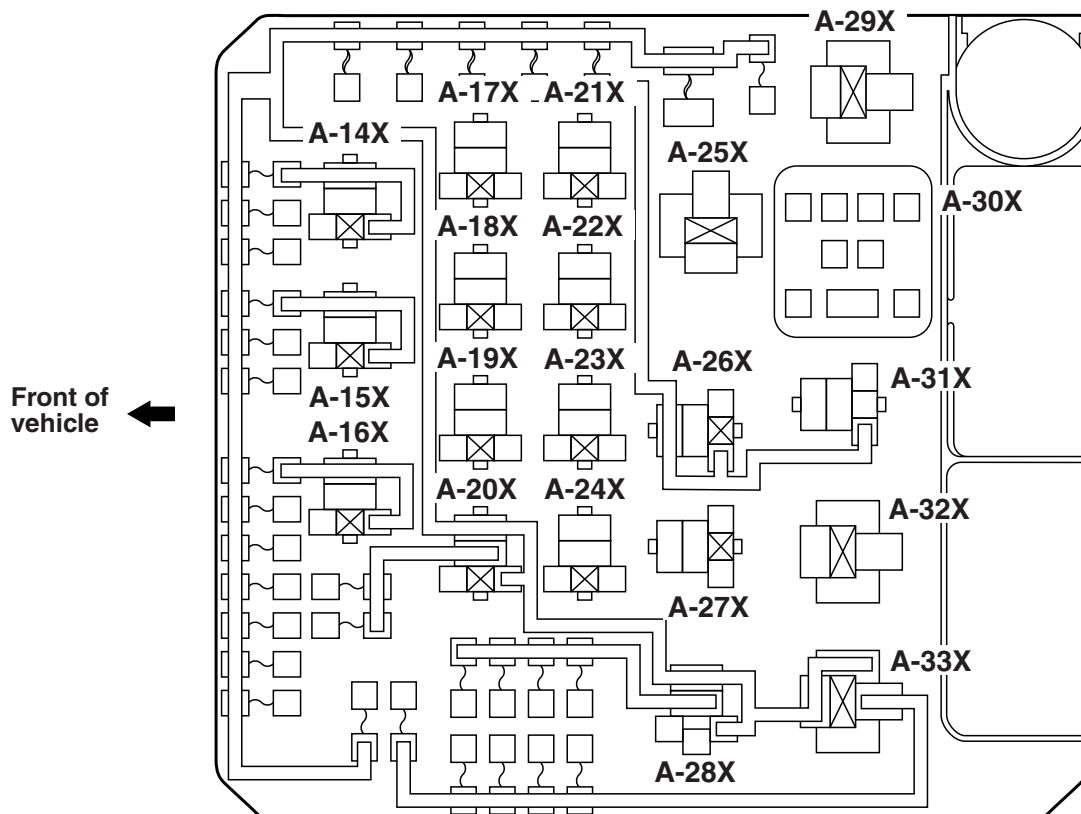
Relay box in engine compartment &lt;2.4L Engine&gt;
