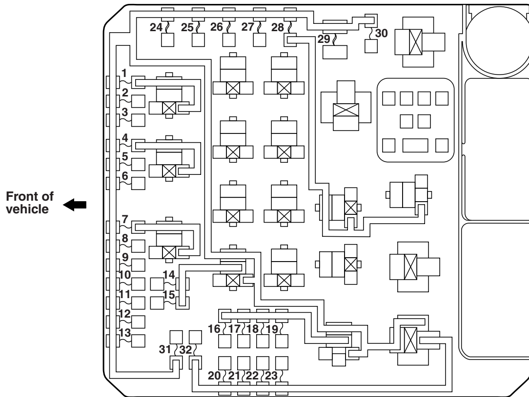
Relay box <2.4L Engine>
