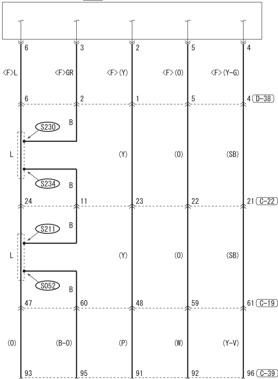
REAR VIEW CAMERA (F-21)
