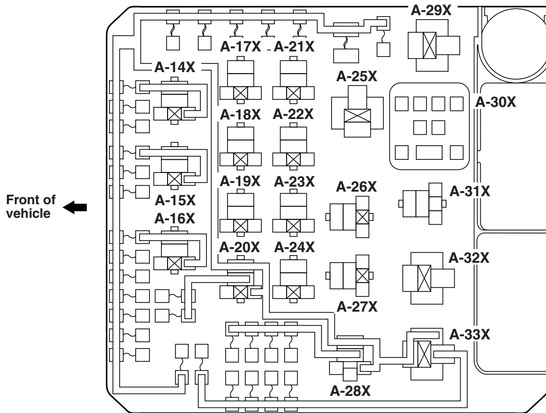
Relay box in engine compartment <3.0L Engine>
