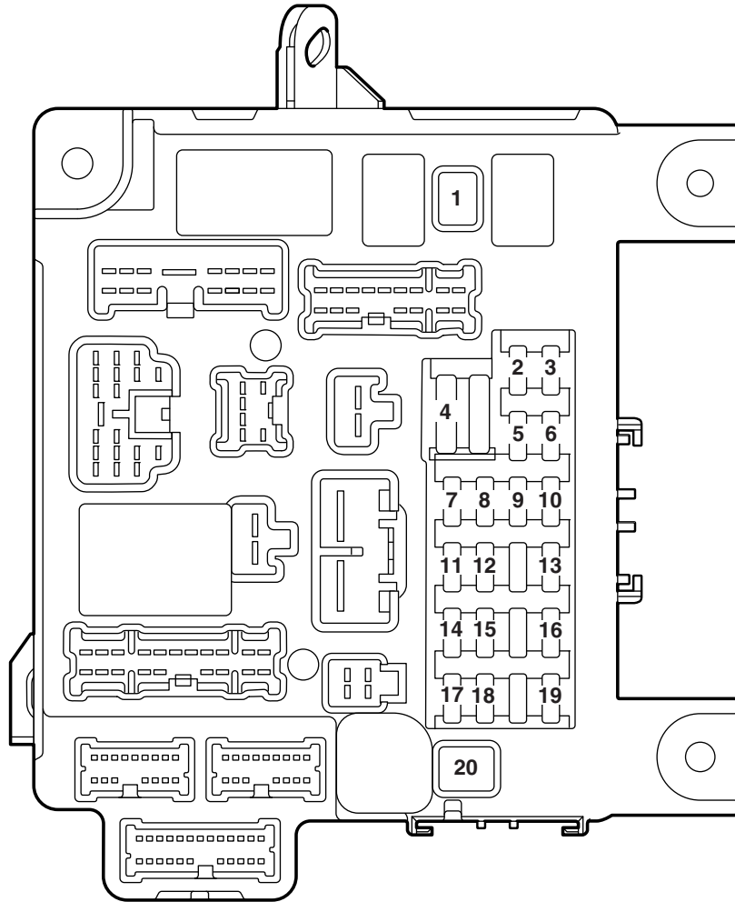
Fuse box in ETACS-ECU
