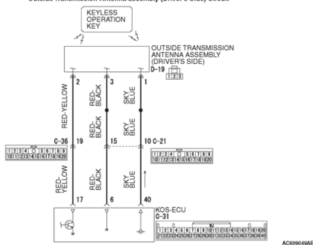
Outside Transmission Antenna assembly (Driver's Side) Circuit
