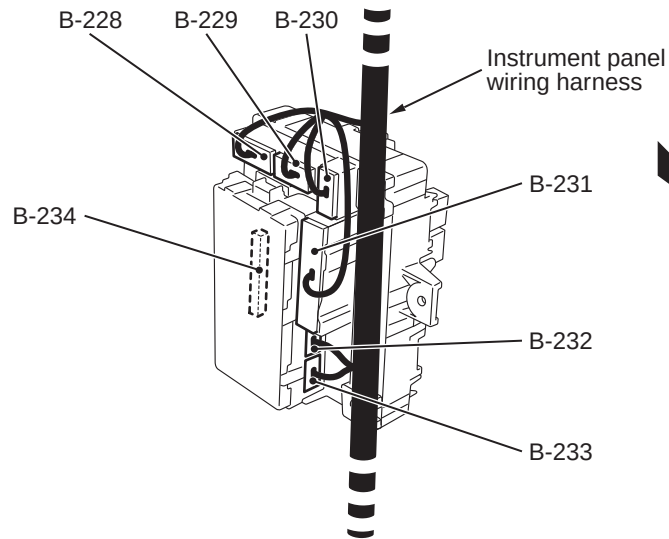
J/B (Rear view)
