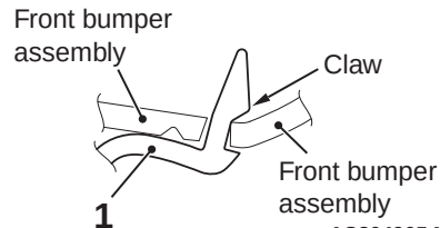
Section D - D
