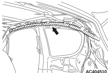
Curtain air bag modules (left and right) <COLT CZ3>
