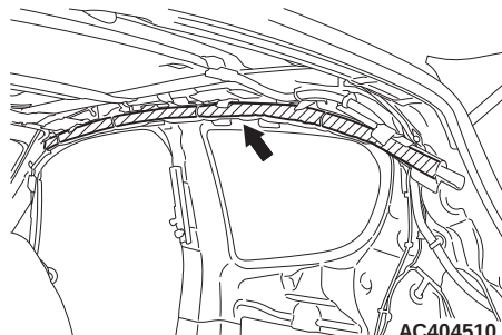
Curtain air bag modules (left and right) <COLT CZ3/CZT>
