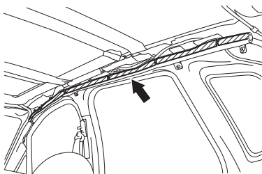
Curtain air bag modules (left and right) <COLT>
