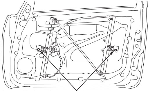
Door window glass mounting screws AC404069AB
