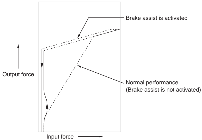
Characteristic diagram
