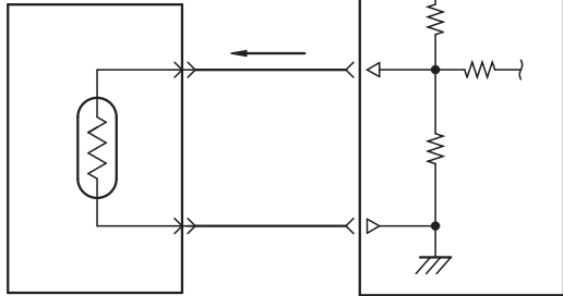
Battery temperature sensor (thermistor)
