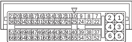
A-34 Harness side connector
