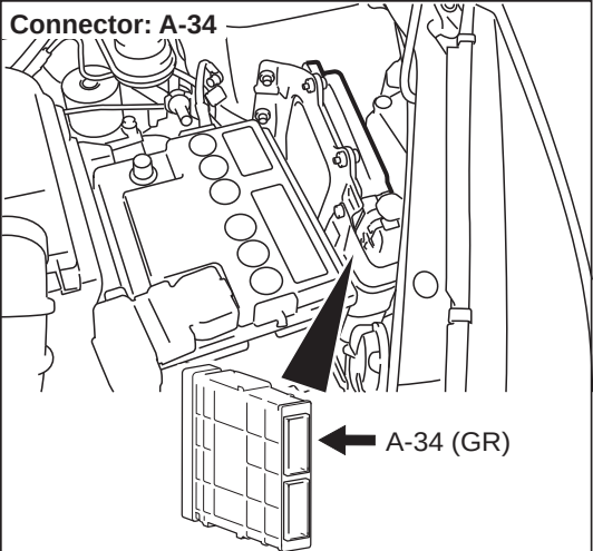
A-34 Harness side connector
