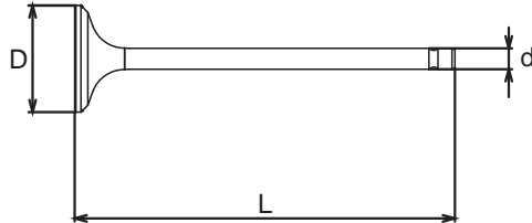
Exhaust
