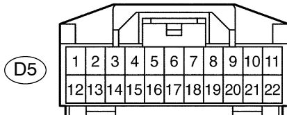
Driver Side Junction Block Wire Harness View:
