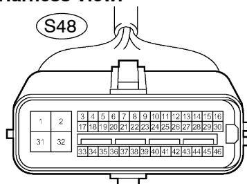
AFS ECU Connector Front View:
