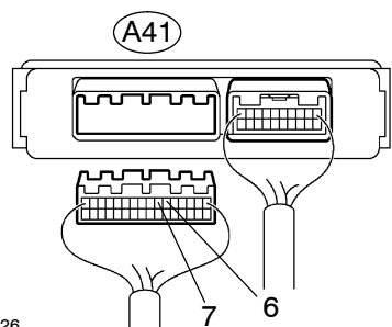
AFS ECU Connector Front View:
