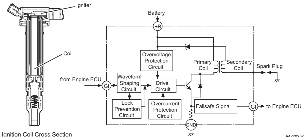
Ignition Coil Cross Section
