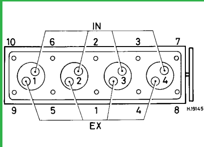
1998 cm 3 , 8V
