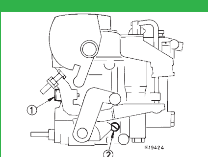
Zenith 32 IF2
